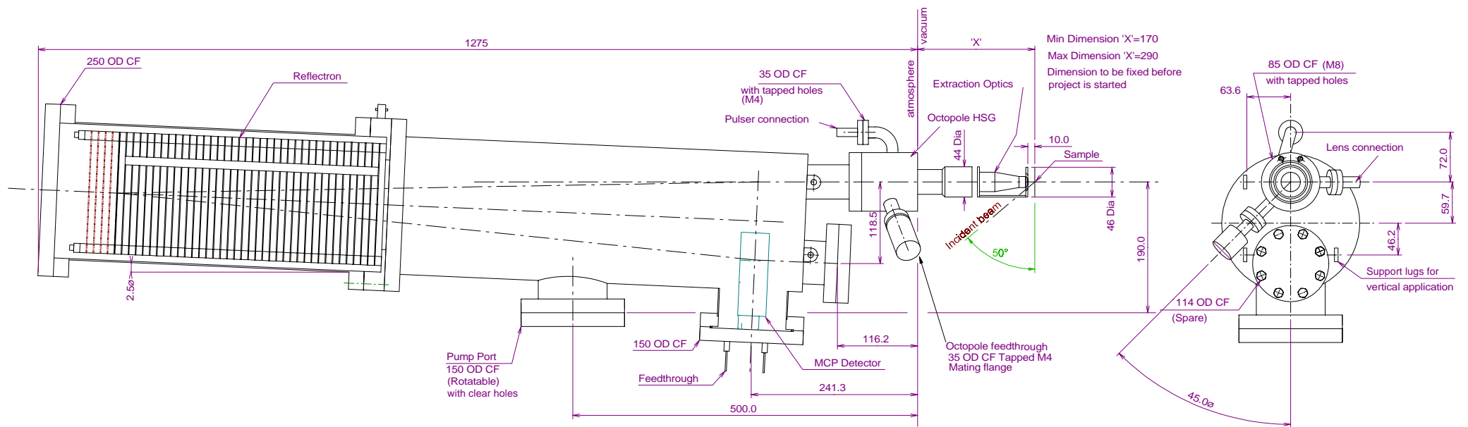
R500 TIME-OF-FLIGHT MASS ANALYSER ASSEMBLY (Copyright Kore Technology Ltd 2000)
